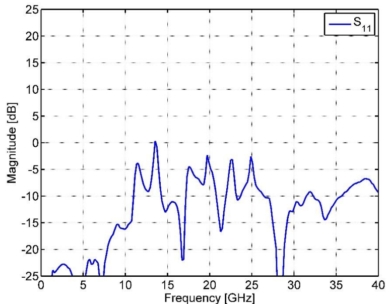
Input reflection
