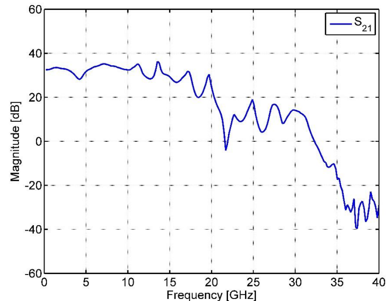
Gain
